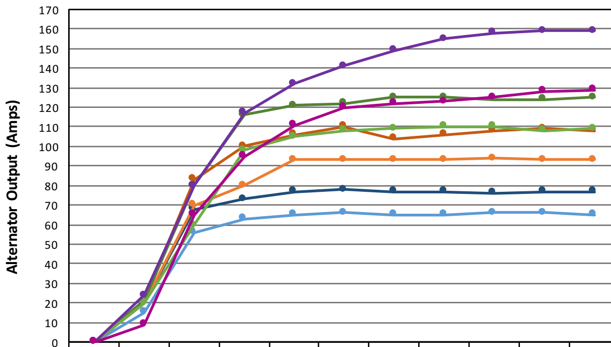
6-Series Alternator Output Comparison 70A, 100A, 120A & 150A (12V) Versions
