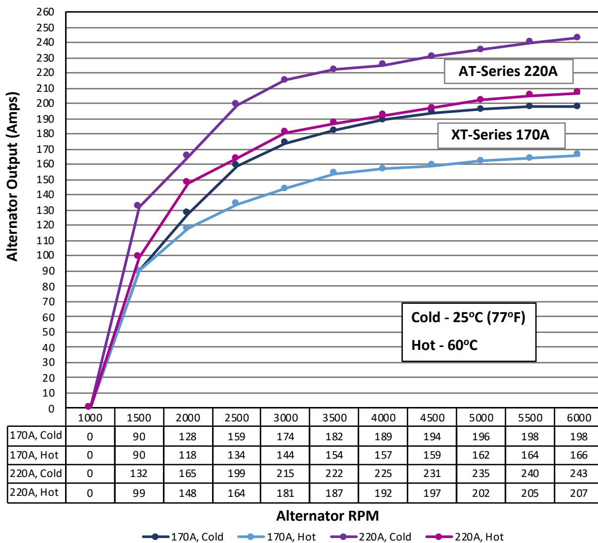
XT-Series & AT-Series Alternator Output Comparison 170A & 220A (12V) Versions
