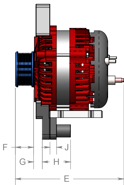
AT-SF-200-XX
