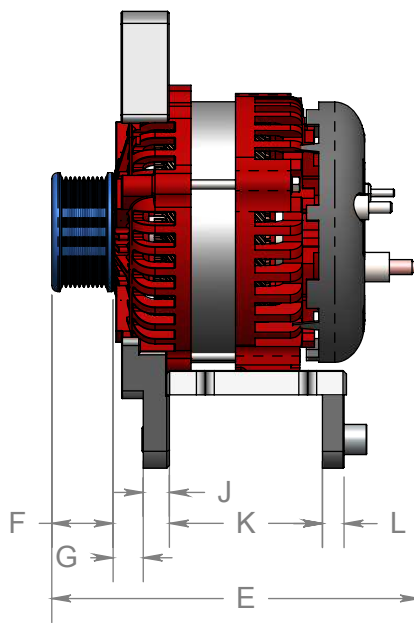
AT-DF-200-XX
